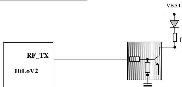
Figure 4: RF TX burst indicator
