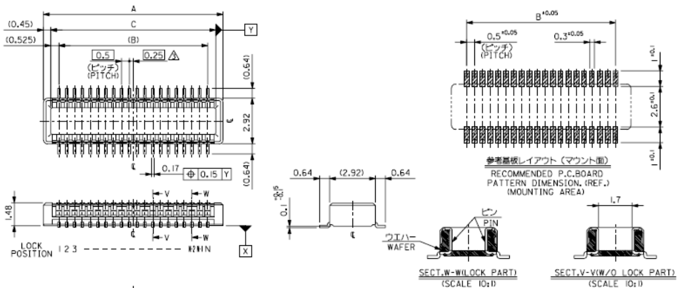
Figure 7: HiLo V2 connector drawing
