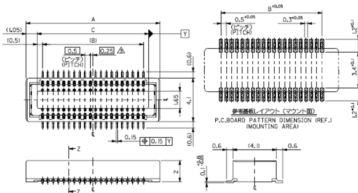
Figure 8: Mother board connector drawing
