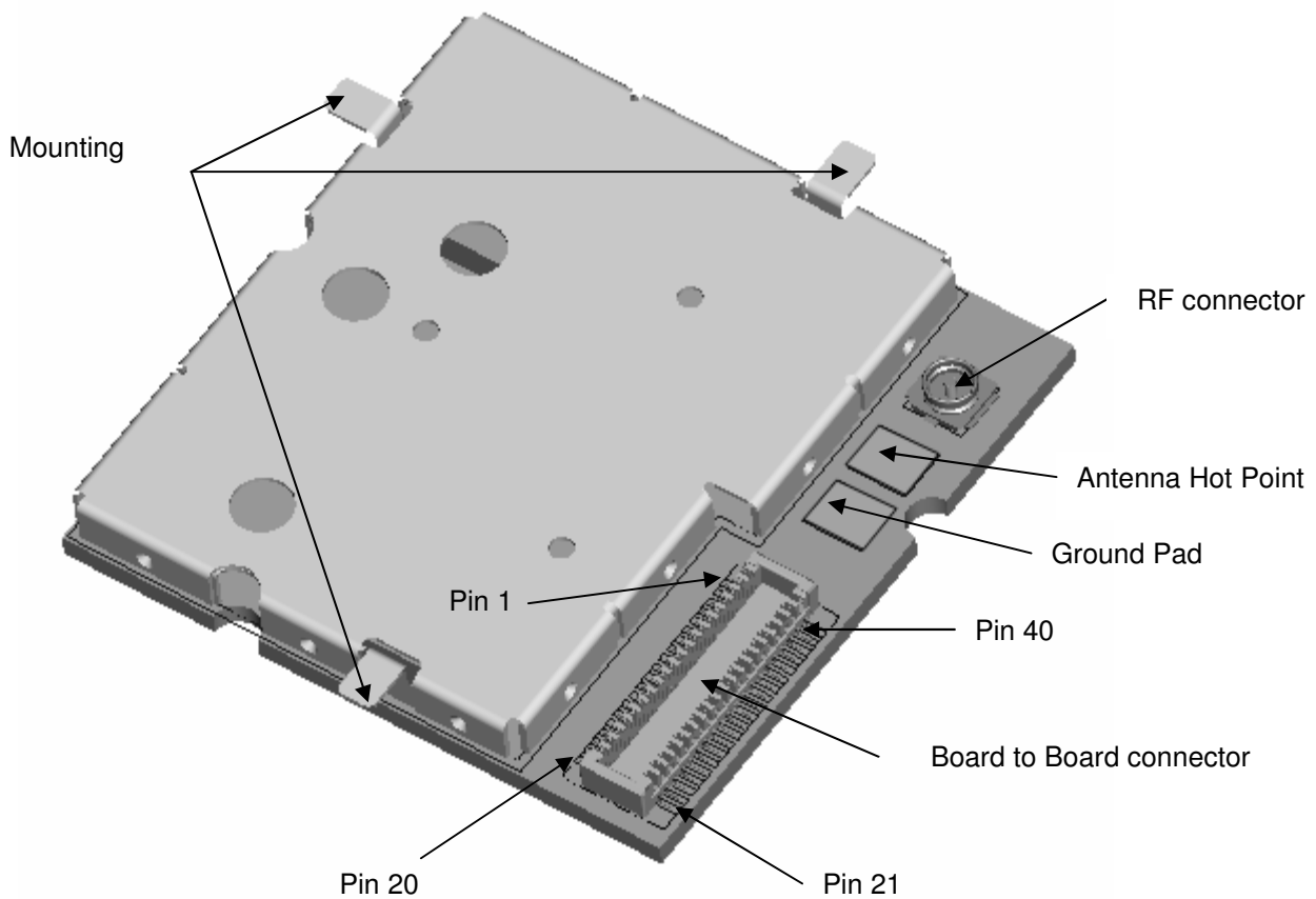
Figure 8: HiLo V2 interface
