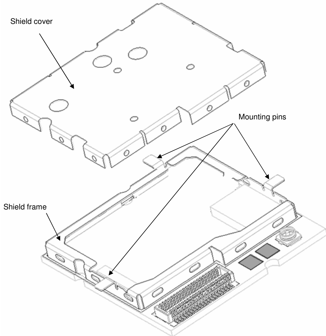
Figure 10: HiLo V2 decomposition
