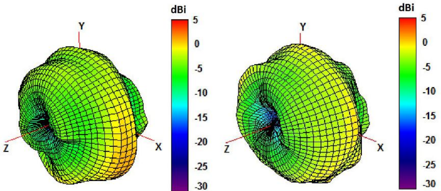
940 and 1750 MHz Radiation pattern
