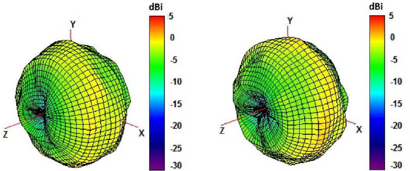
1850 and 1950 MHz Radiation pattern
