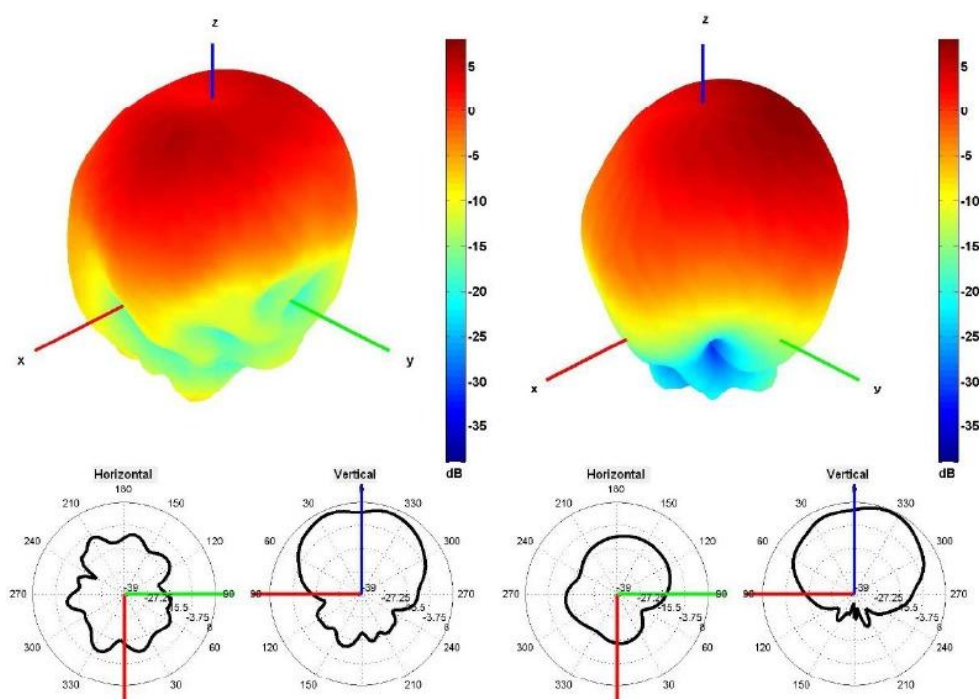
2100 and 2600 MHz Radiation pattern
