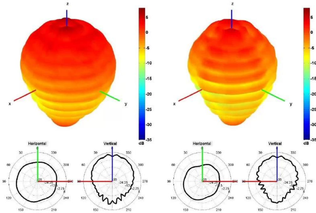
1561 and 1575 MHz Radiation pattern
