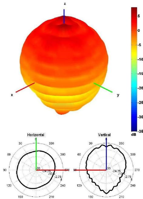
1602 MHz Radiation pattern
