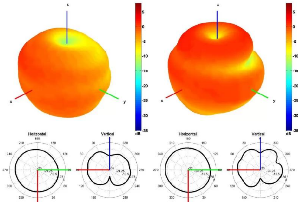
2360 and 2660 MHz Radiation pattern
