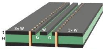
Coplanar Waveguide Grounded (CPW-G)
