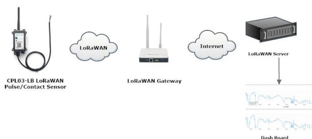
CPL03-LB in LoRaWAN Network
